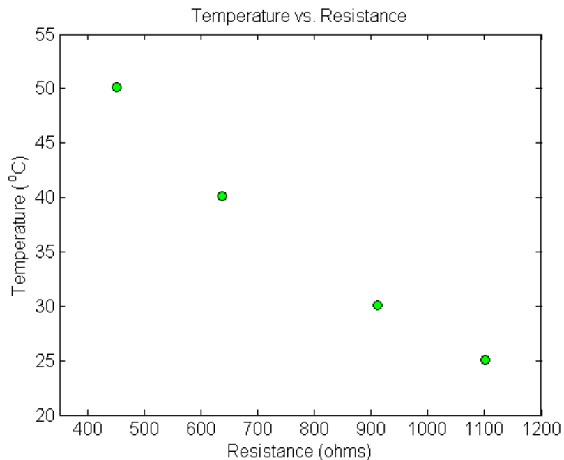
Figure 1 Resistance vs. temperature.
